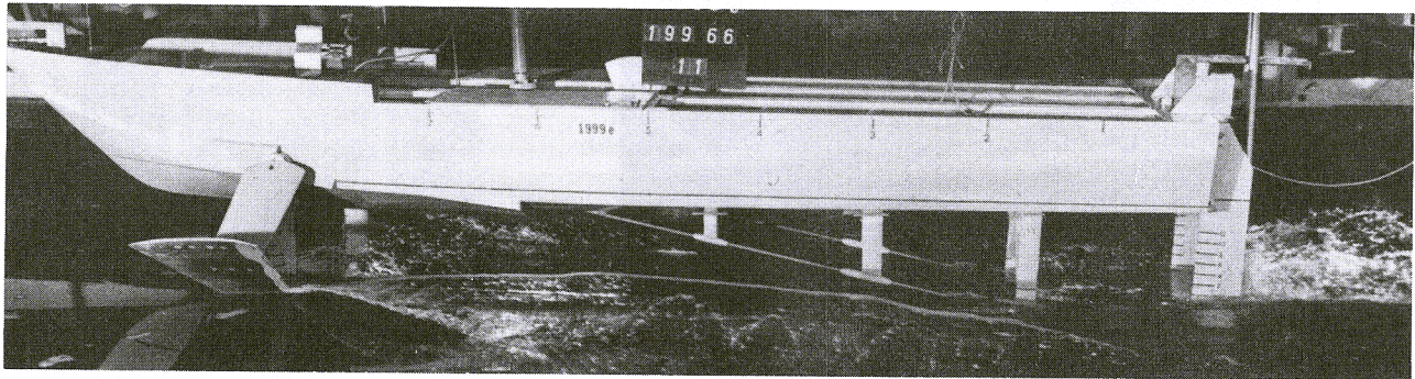
Figure 3.4.6 - Foilborne Mode
