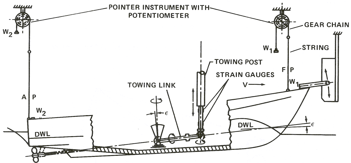
Figure 3.2.5 - Towing Setup for Resistance Tests
