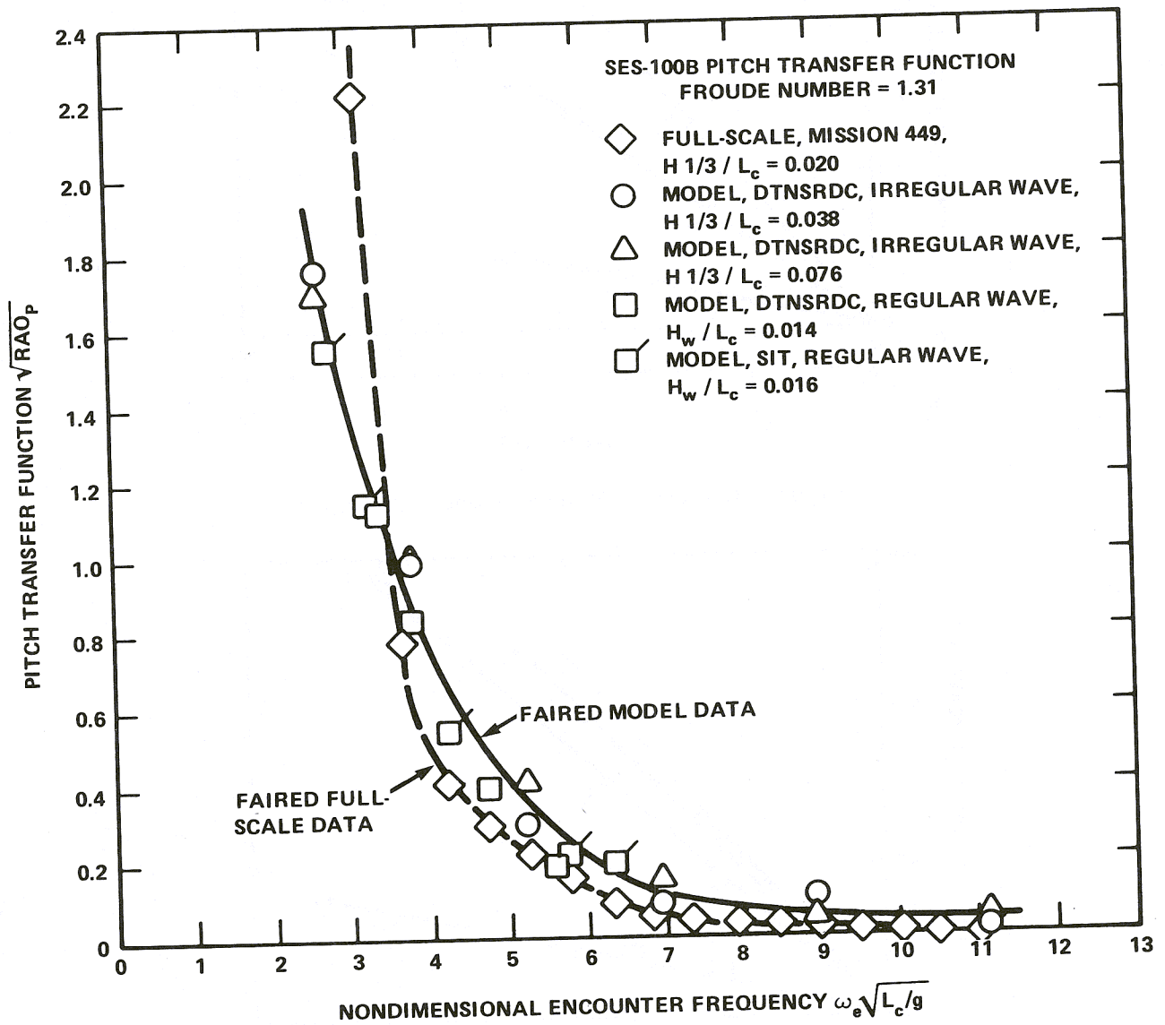
Figure 3.5.19 - SES-100B Model and Full-Scale Pitch Response Comparison at a Froude Number of 1.31
