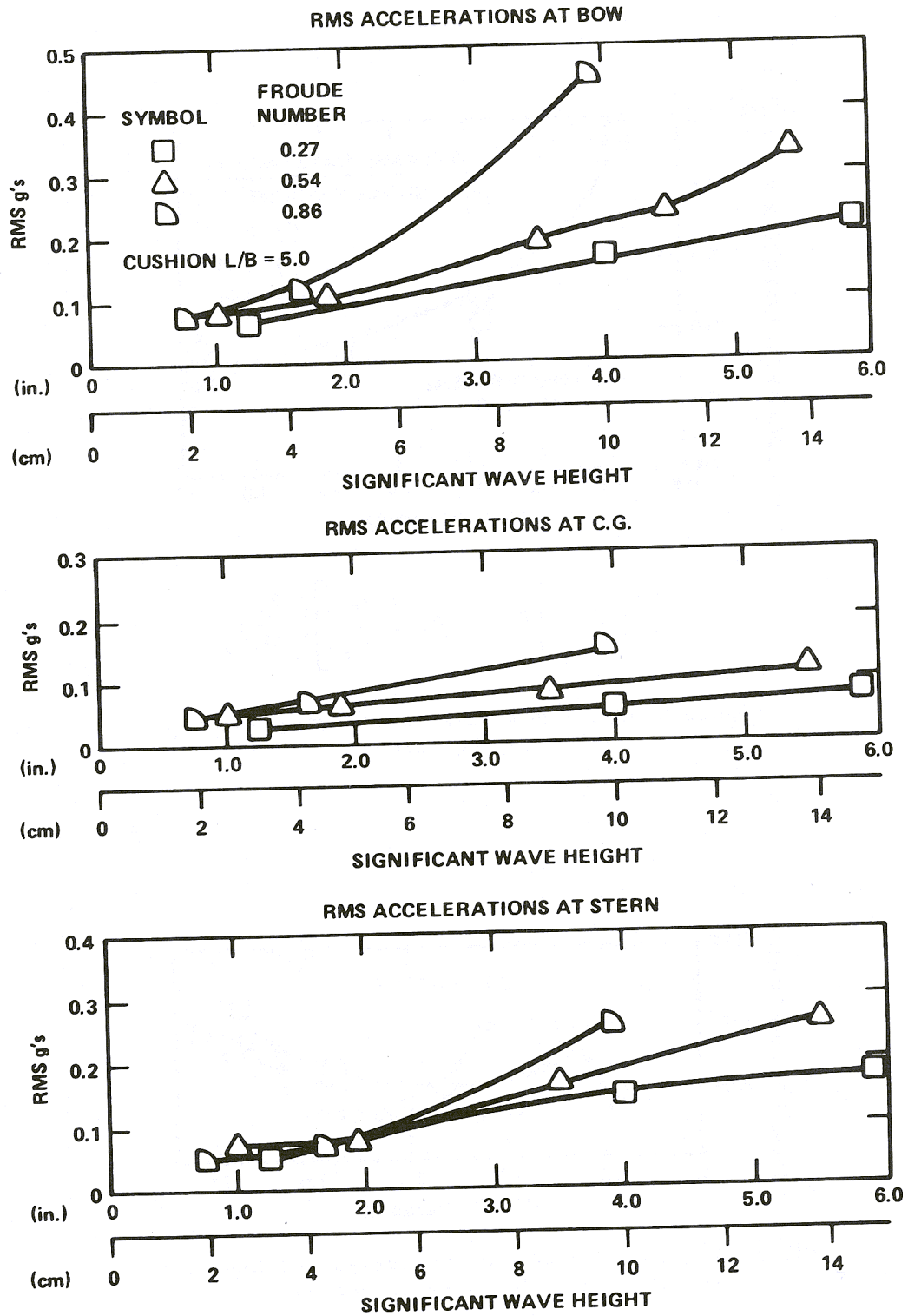
Figure 3.5.14 - Root Mean Square Accelerations for Various Significant Wave Heights and Froude Numbers
