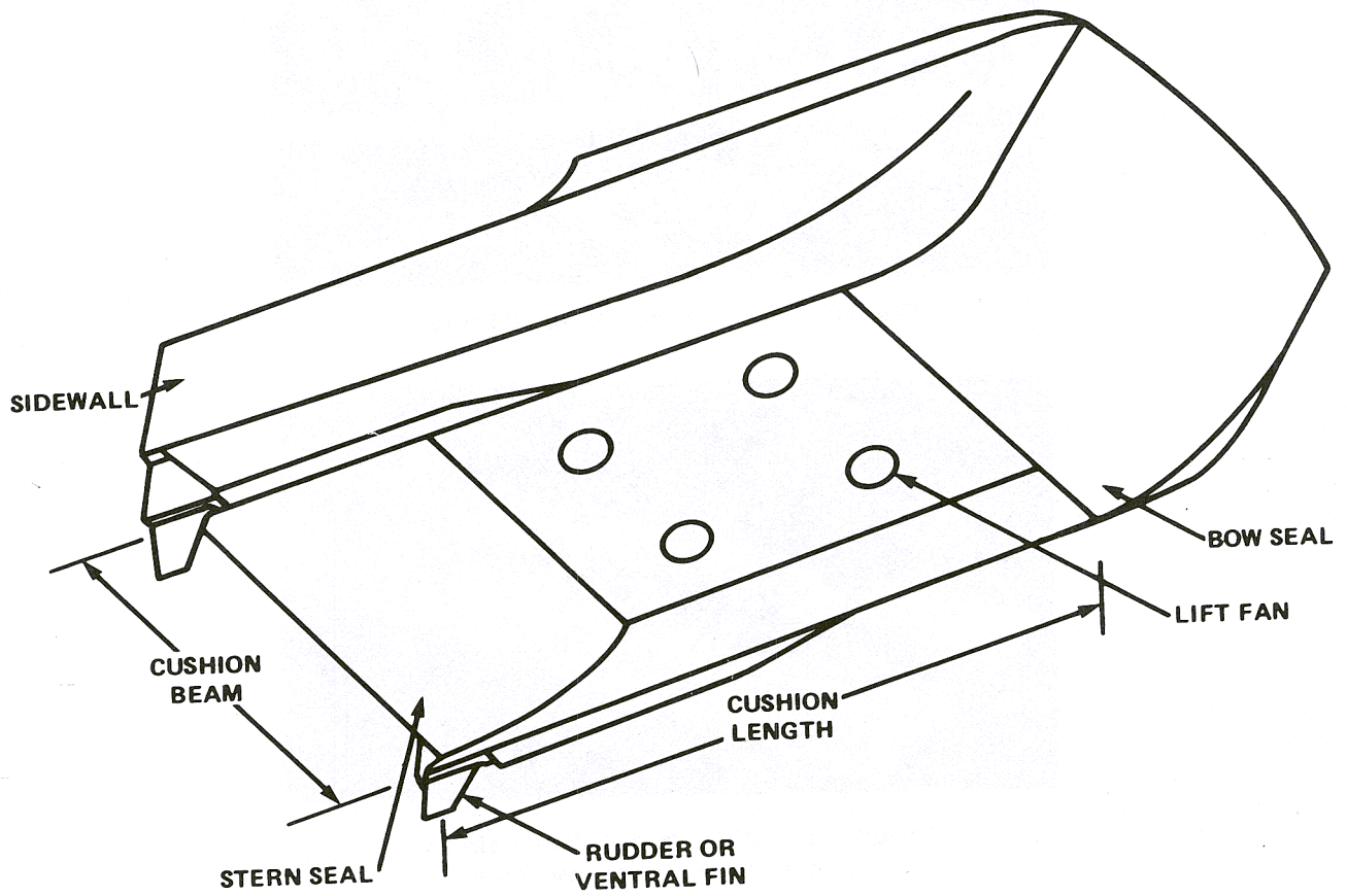
Figure 3.5.1 - Surface Effect Ship
