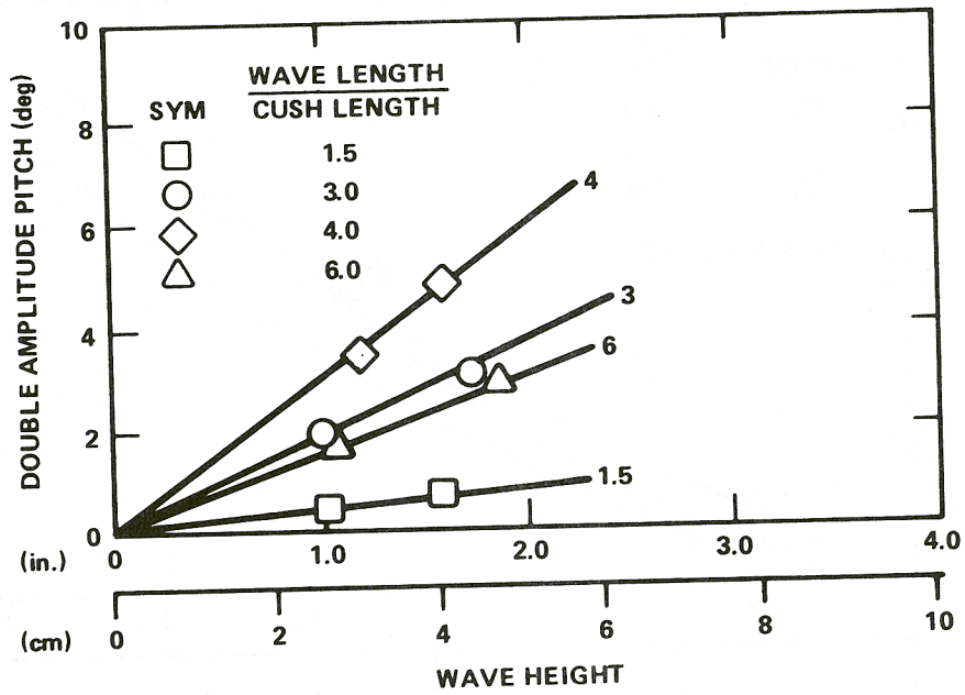
Figure 3.5.17a - Froude Number = 1.72
