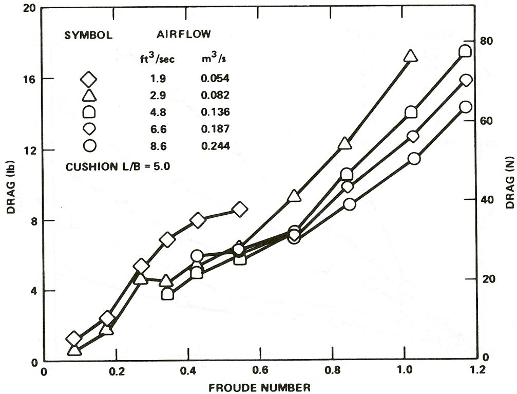
Figure 3.5.6 - Drag Variations Due to Total Airflow Rate
