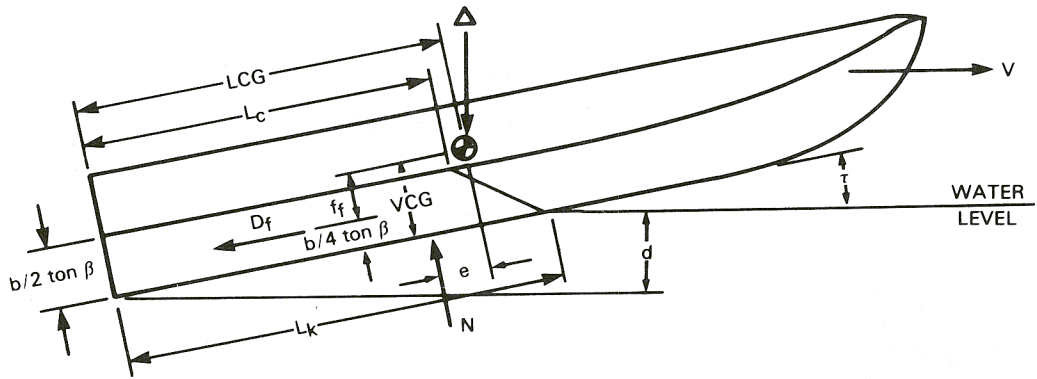
Figure 3.3.7a- Forces and Moments on a Planing Surface
