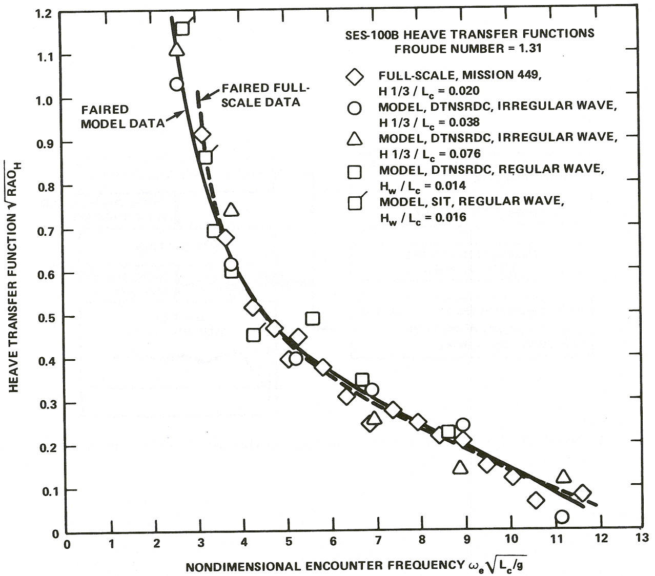
Figure 3.5.20 - SES-100B Model and Full-Scale Heave Response Comparison at a Froude Number of 1.31
