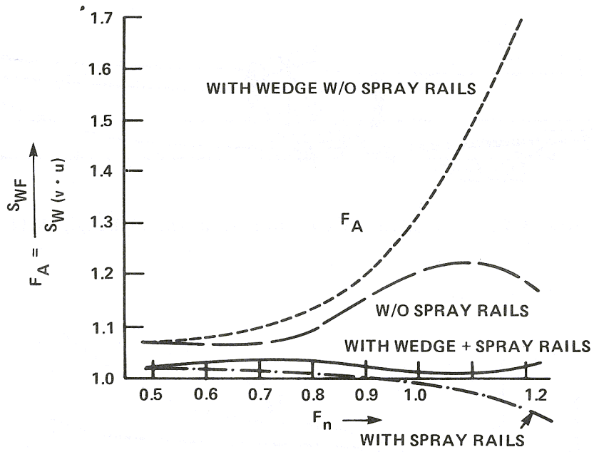
Figure 3.2.3 - Change of Wetted Area
