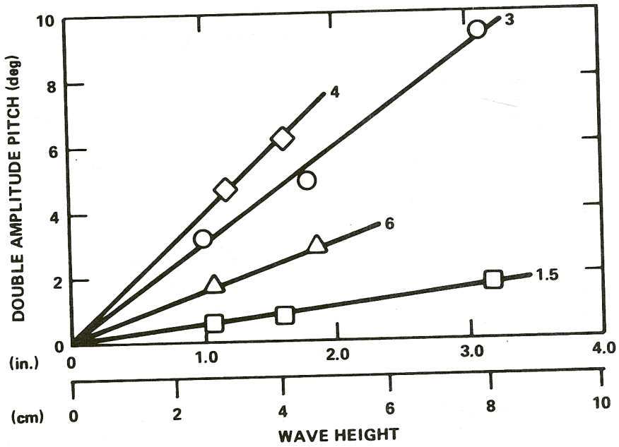
Figure 3.5.17b - Froude Number = 1.28
