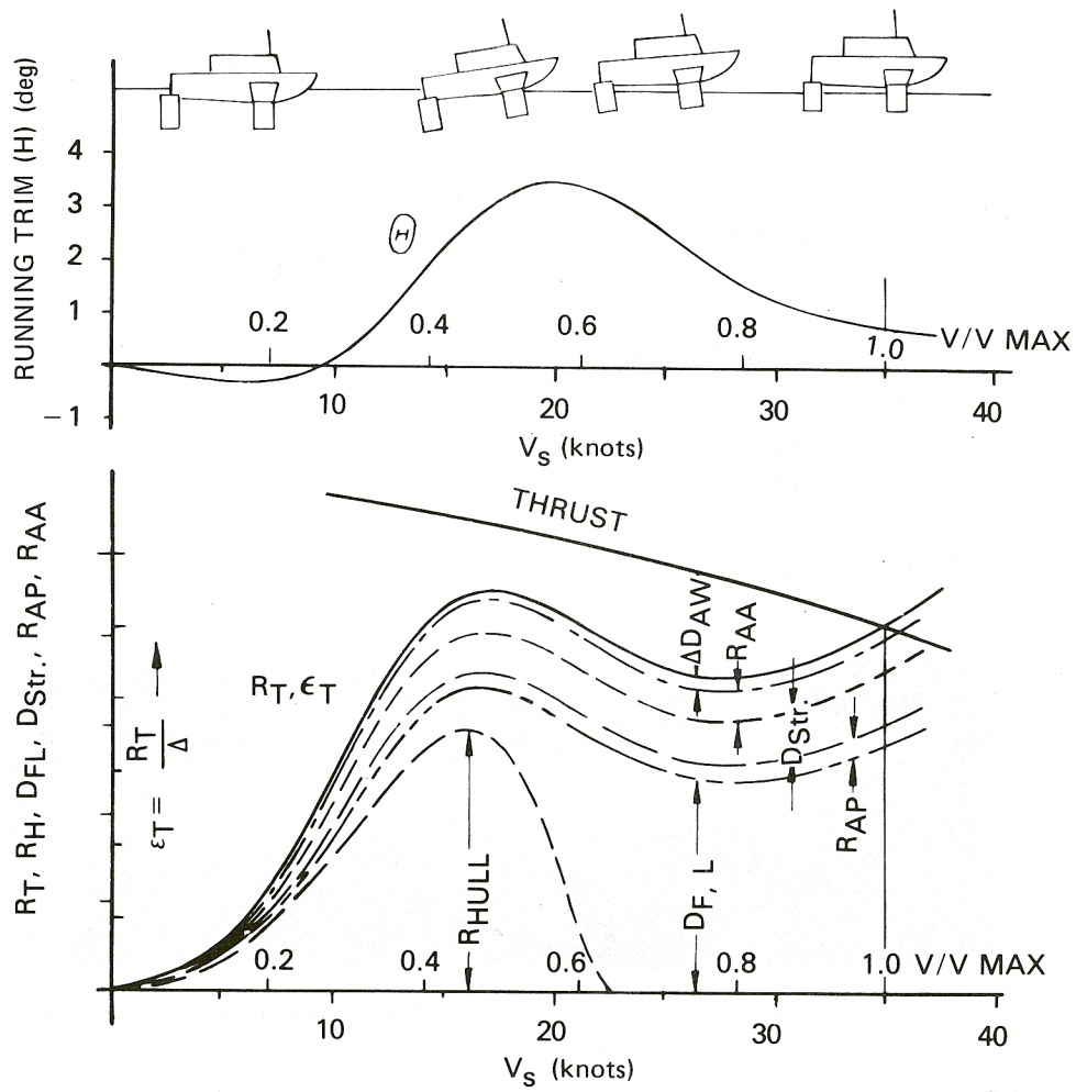
Figure 3.4.5 - Distribution of Resistance Components, Running Trim, Attitude
