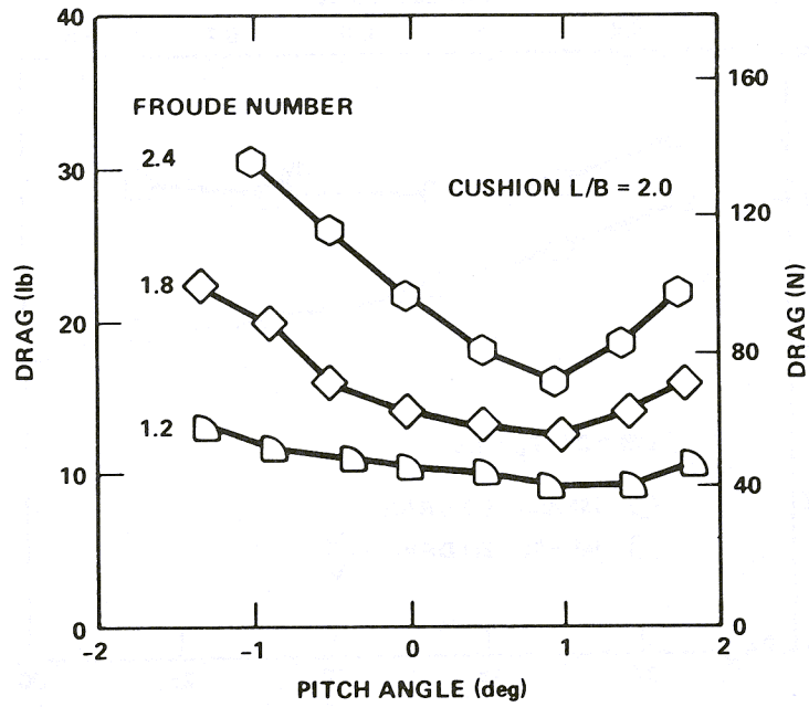
Figure 3.5.5 - Drag Variations with Pitch Angle and Froude Number
