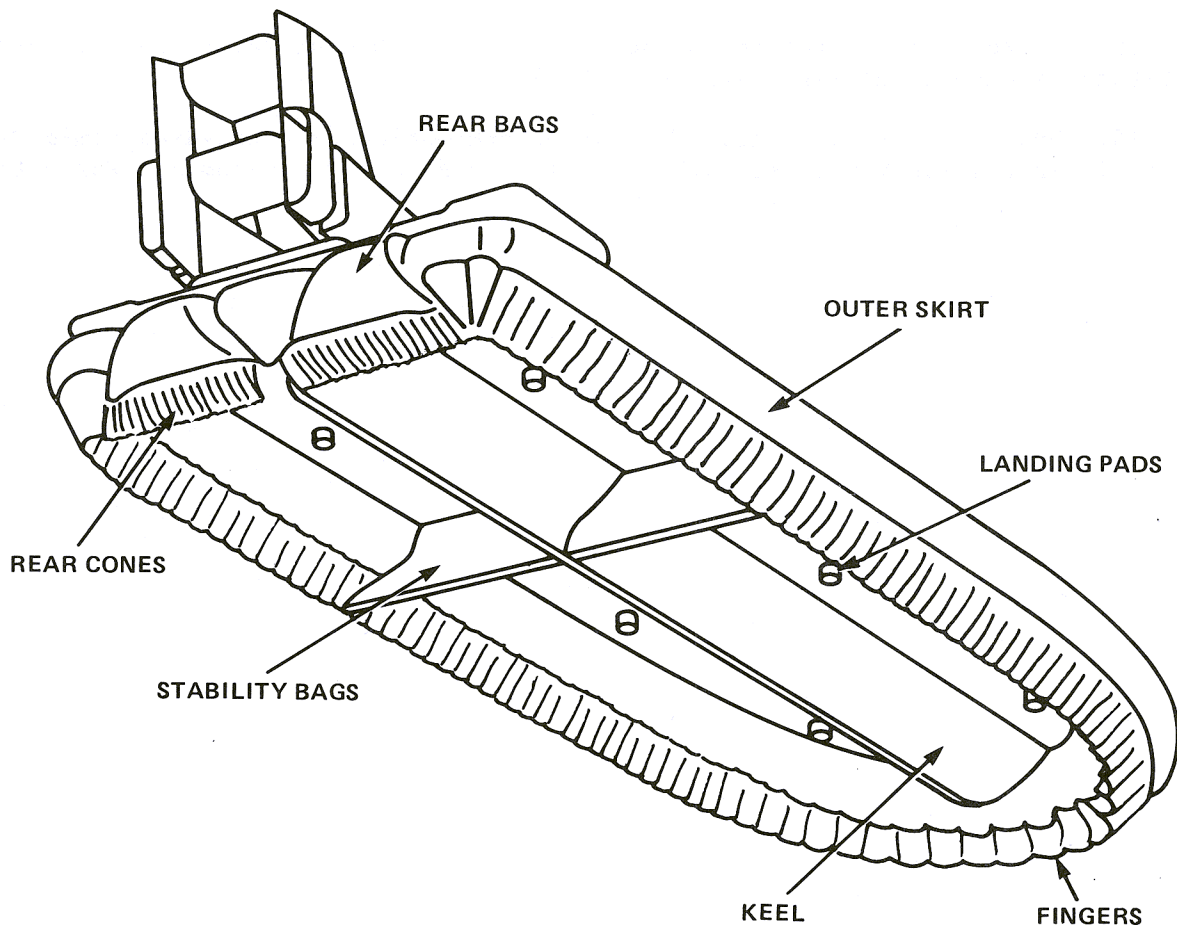
Figure 3.6.1 - Typical Small ACV Fitted with BHC Type Peripheral Skirt
