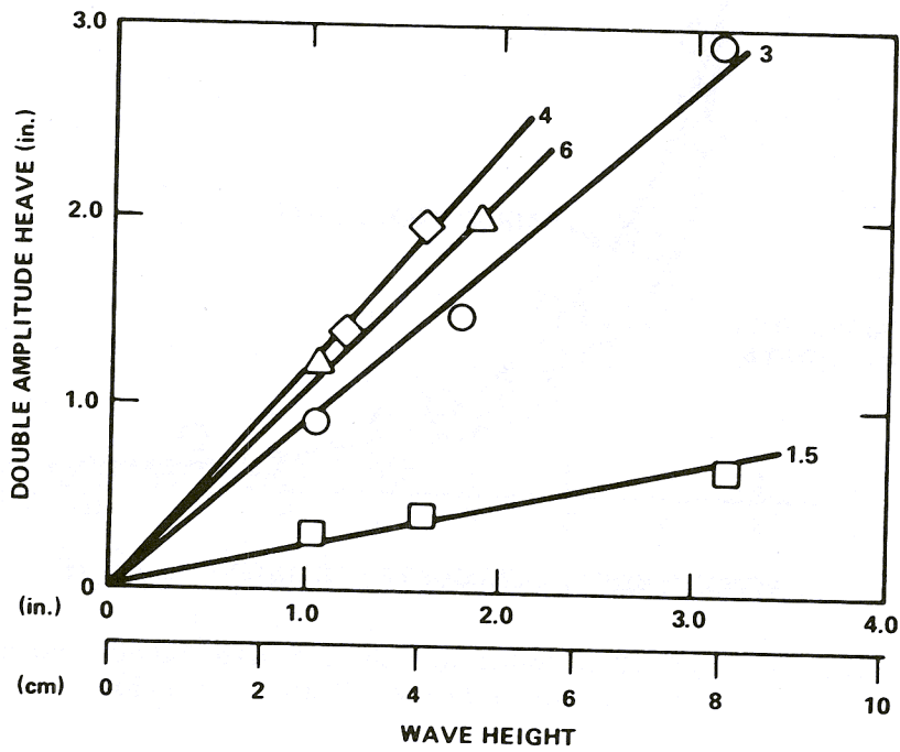
Figure 3.5.18b - Froude Number = 1.28
