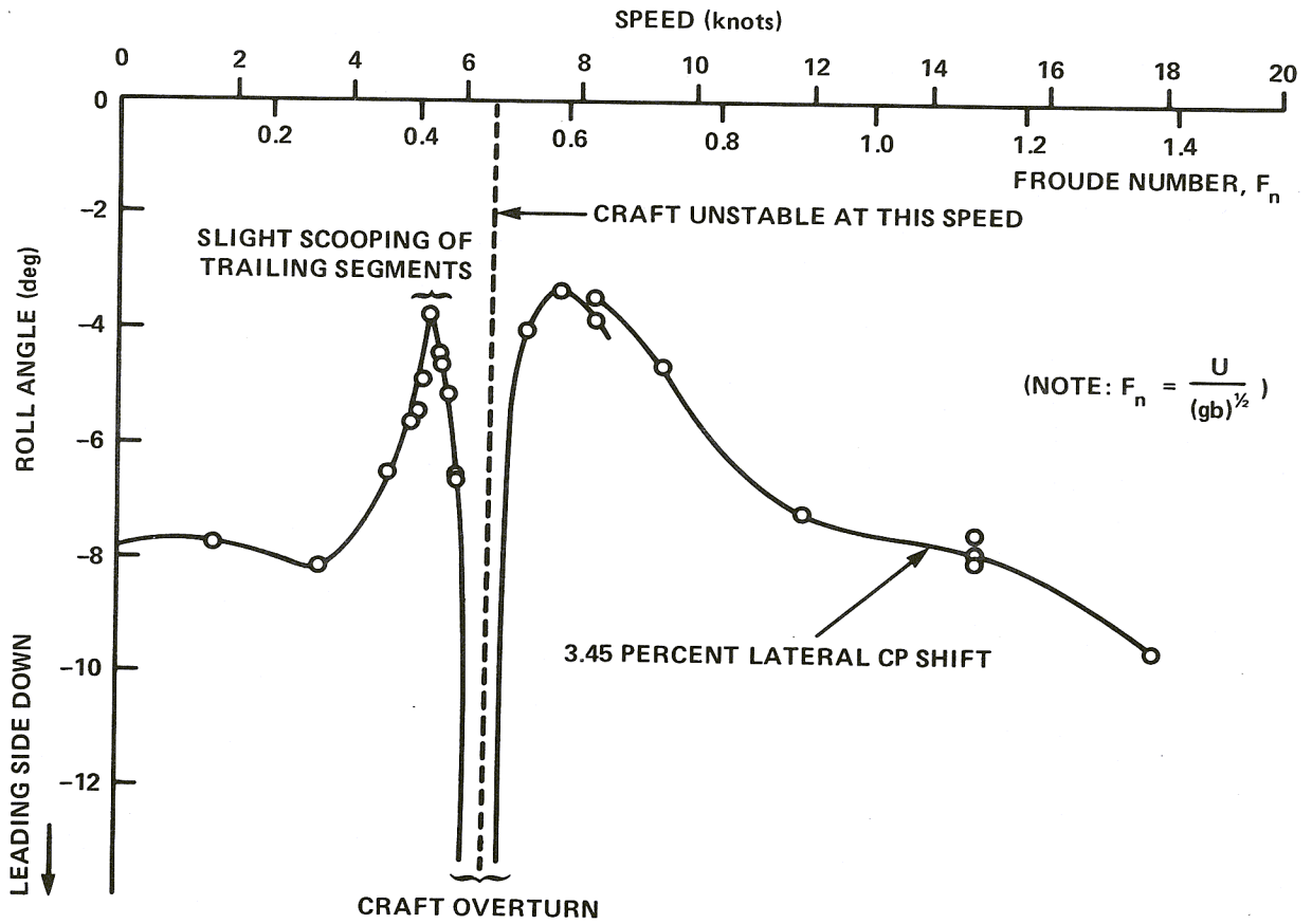
Figure 3.6.10 - Example of Critical Speed Definition from Model Tests
