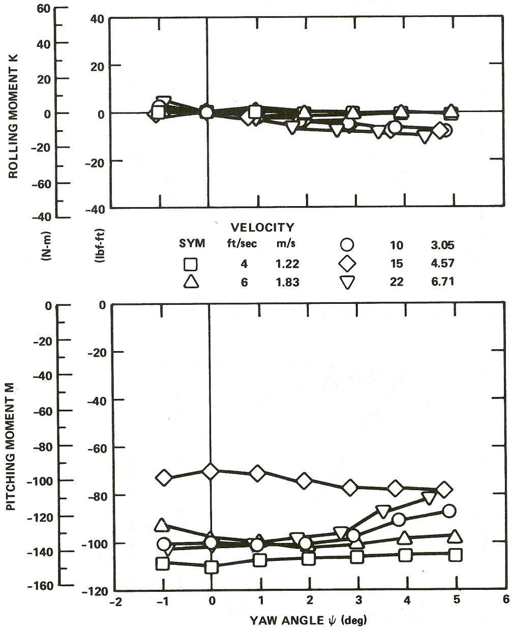
Figure 3.5.23b - Rolling Moment and Pitching Moment Data
