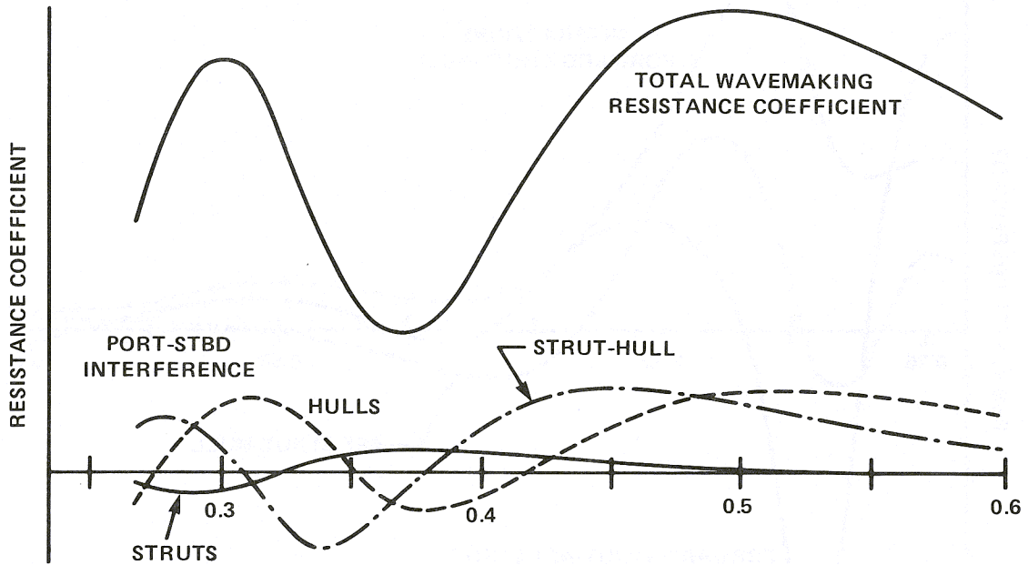
Figure 3.1.2 - Typical Wavemaking Resistance Coefficients versus Froude Number Single-Strut-per-Hull SWATH
