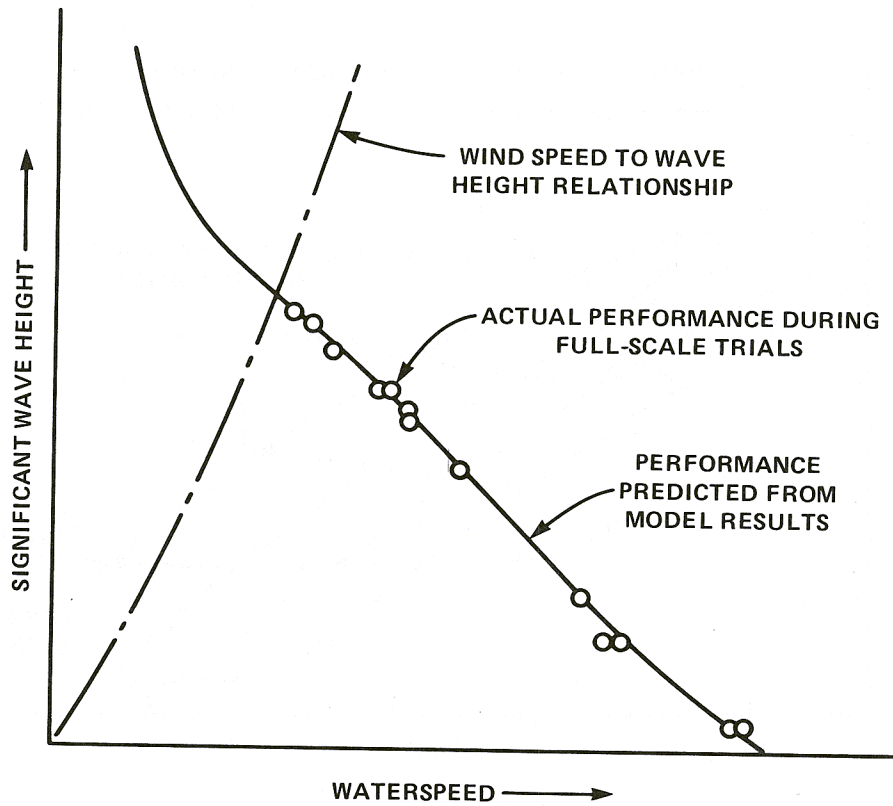
Figure 3.6.9 - Actual and Predicted into Wind Waterspeed Performance
