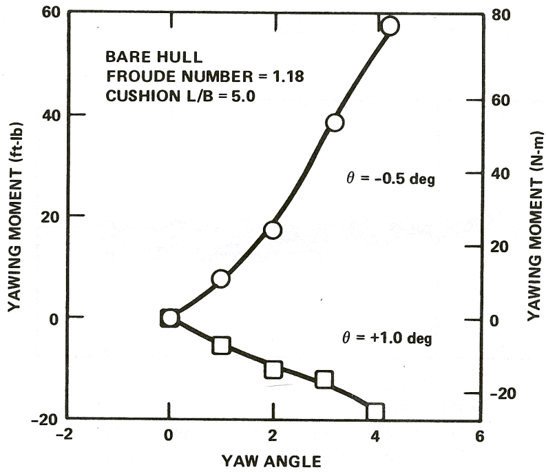
Figure 3.5.24a - Pitch Attitude Effect on Yaw Moment
