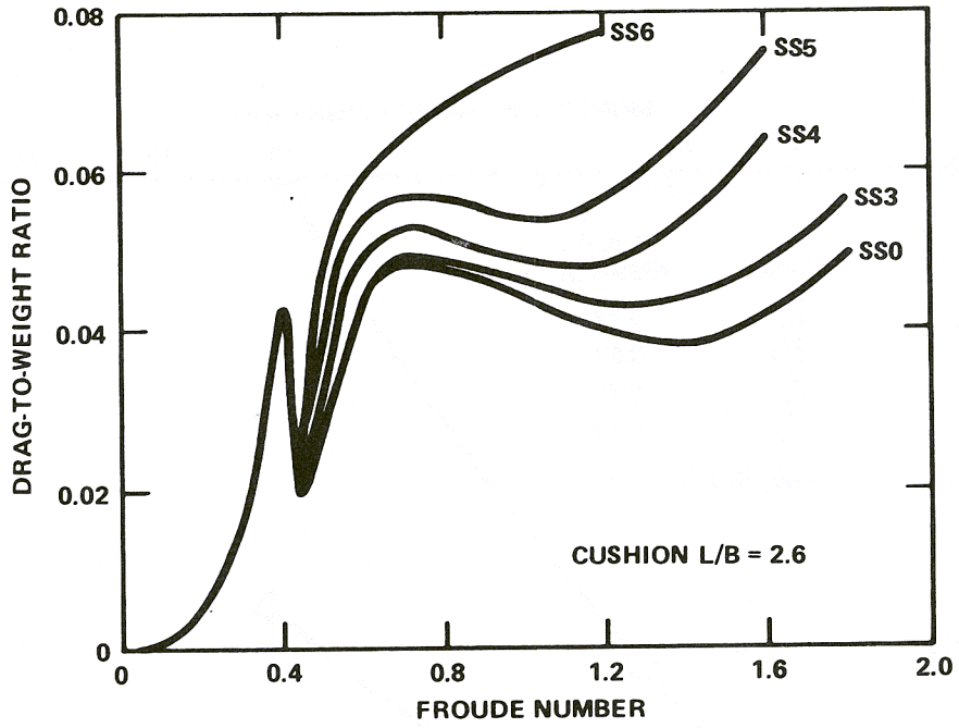
Figure 3.5.10 - State of Sea Effect on Drag
