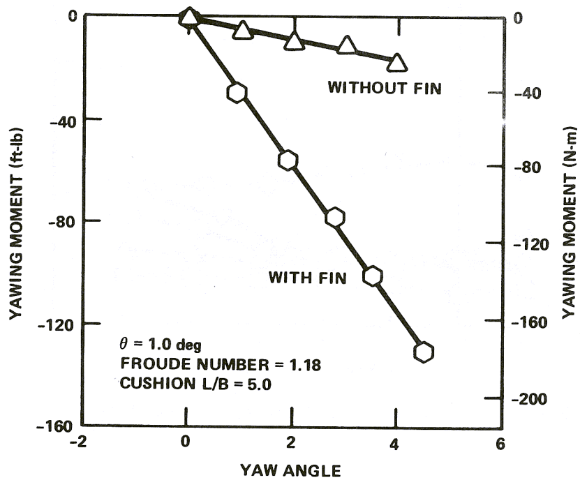
Figure 3.5.24b - Ventral Fin Effect on Yaw Moment
