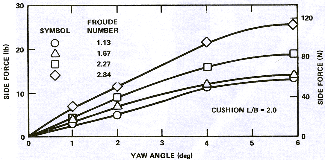
Figure 3.5.26 - Side Force Nonlinearities
