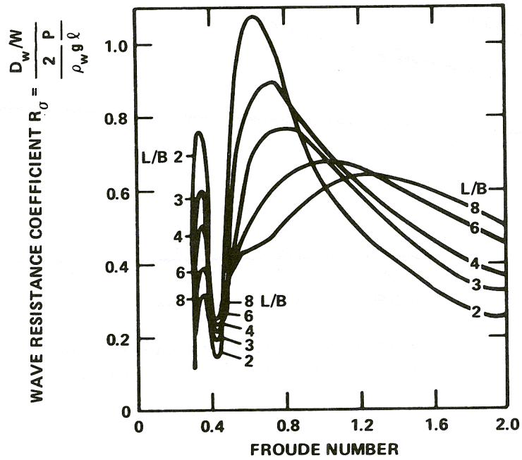
Figure 3.5.11 - Doctors' Wave Resistance Coefficient
