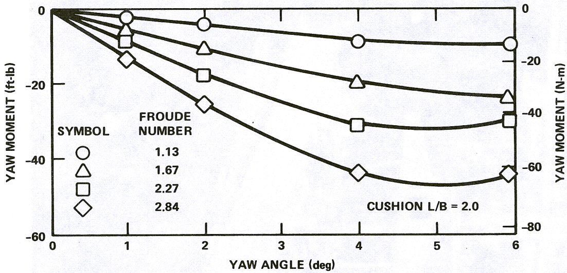
Figure 3.5.25 - Yaw Moment Nonlinearities
