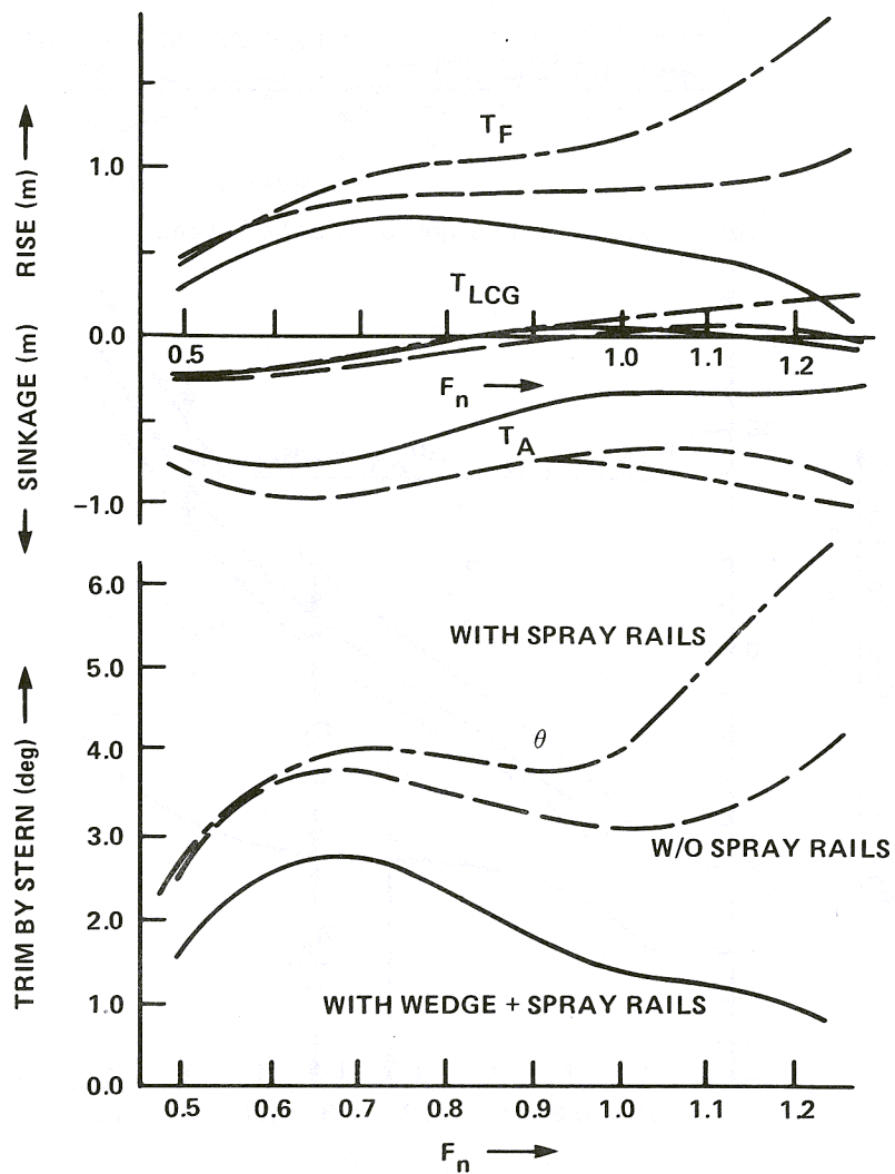
Figure 3.2.2 - Trim Variations
