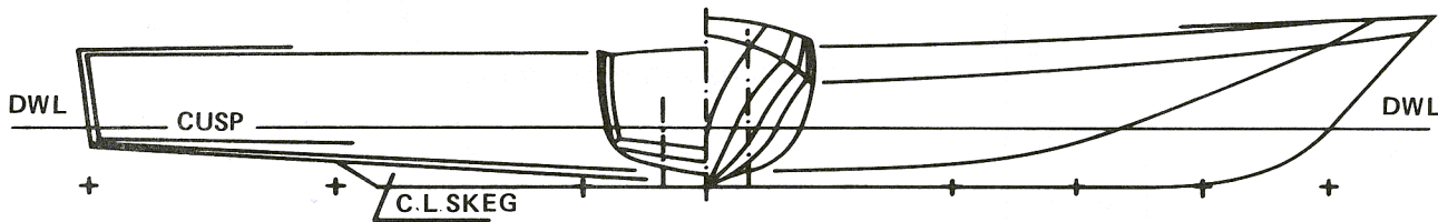
Figure 3.2.1 - Typical Body Plan of a Round-Bilge Hull
