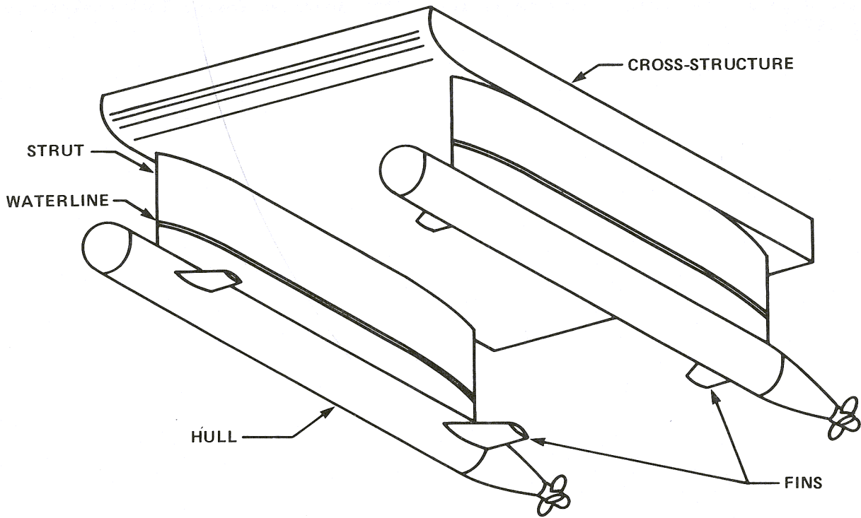
Figure 3.1.1 - SWATH Configuration and Nomenclature
