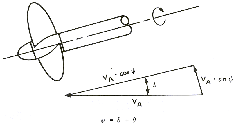
Figure 3.2.6 - Velocities at Propeller in Oblique Flow
