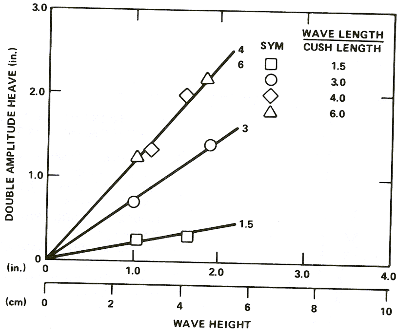
Figure 3.5.18a - Froude Number = 1.72
