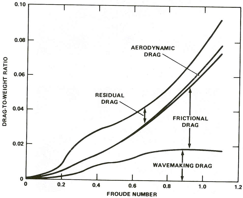
Figure 3.5.3b - Cushion L/B = 6.0
