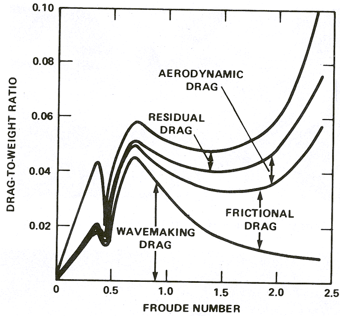
Figure 3.5.3a - Cushion L/B = 2.0
