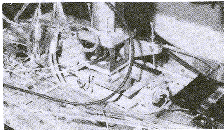
Figure 3.5.2f - Model Tow Post, Force Gage, Gimbal, and Pitch and Roll Potentiometers
