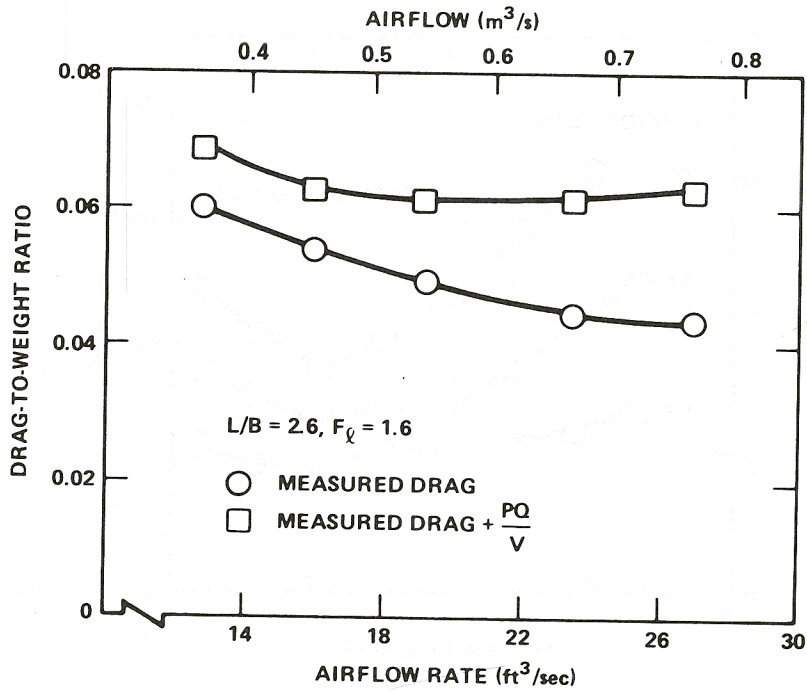
Figure 3.5.7 - Effect of Airflow Rate on Drag
