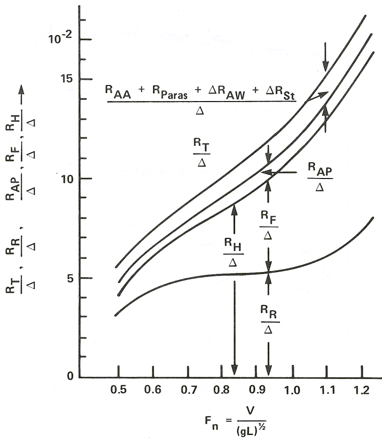
Figure 3.2.4 - Drag-Weight Ratios of Full-Scale Round-Bilge Hull
