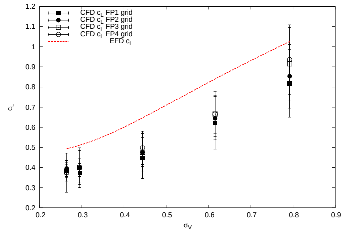
Figure 22: Lift Coefficient predictions at different cavitation indexes \sigma_V . Dots: numerical results obtained with different mesh resolutions; curve experimental measurements. Circular Arc geometry at Re = 6.19E5 , \alpha = 10 \text{ deg} .
