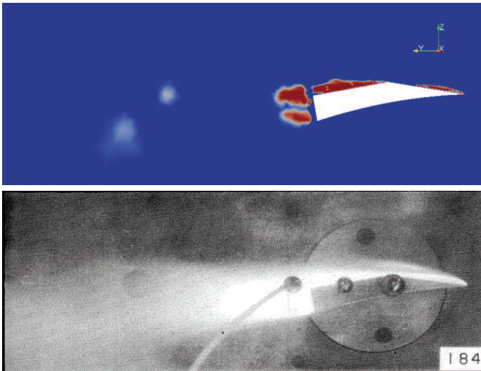
(c) \sigma_V = 0.792 Top pannel CFD, bottom pannel EFD
