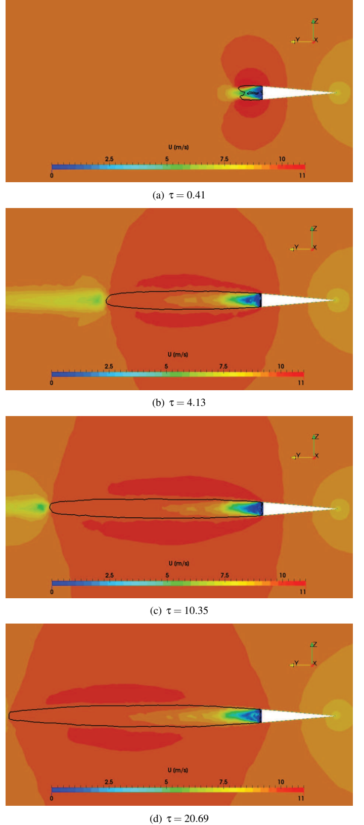
Figure 11: Unsteady flow solution: velocity Contours at cavitation index \sigma_V = 0.141 at different non-dimensional time instants /\tau . Last time step corresponds to the steady state solution. In black VoF = 0.5
