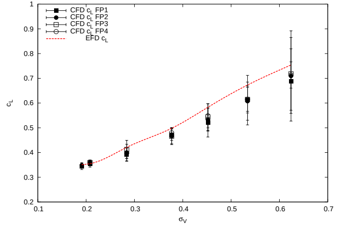
Figure 16: Lift Coefficient predictions at different cavitation indexes \sigma_V . Dots: numerical results obtained with different mesh resolutions; curve experimental measurements. Flat Plate geometry at Re = 4.52E5 , \alpha = 7 \text{ deg} .
