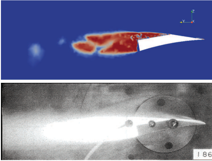
(b) \sigma_V = 0.444 Top pannel CFD, bottom pannel EFD
