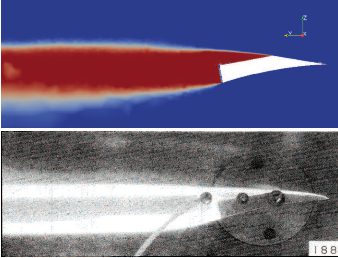
(a) \sigma_V = 0.264 Top pannel CFD, bottom pannel EFD
