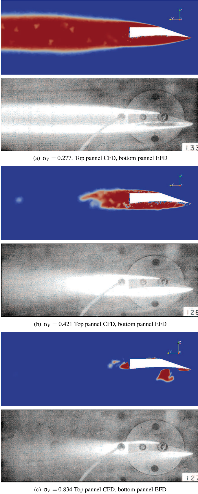
Figure 20: Comparison of the cavity shape predicted by the proposed numerical model and the experimental observation. Circular arc profile at \alpha = 0 \text{ deg} . \tau = 30
