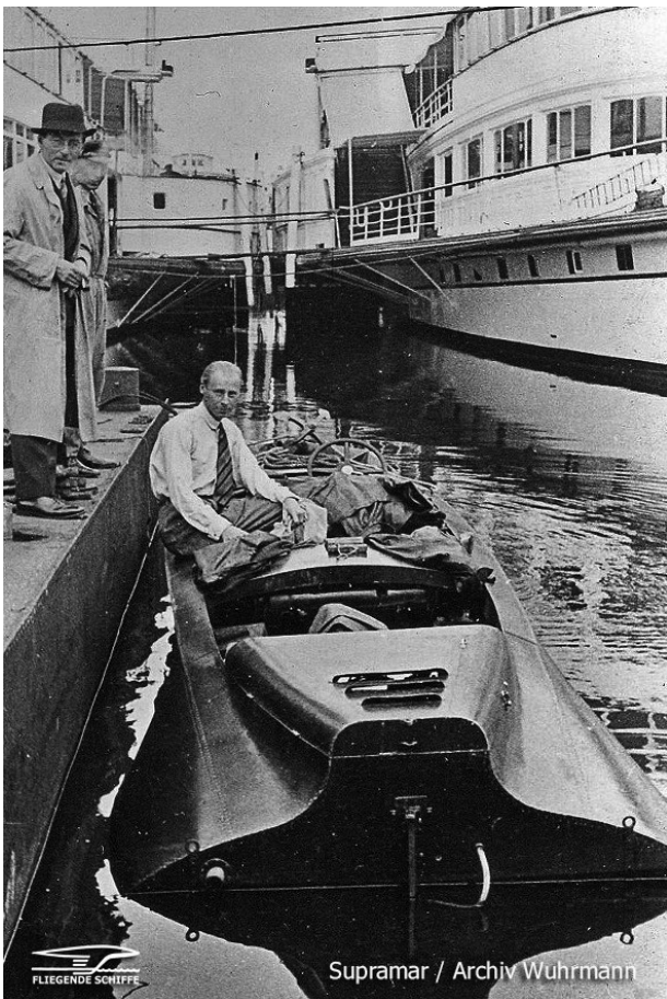
Schertel Prototype (top) Prototypes #3 (middle) and #4 (bottom)
